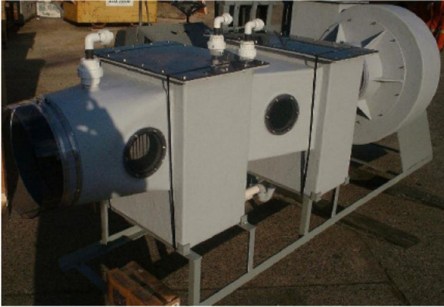
2 bank Scrubber and Fan Systems, 3 micron
